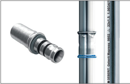
↑ Geberit Mapress with stainless steel adapters
